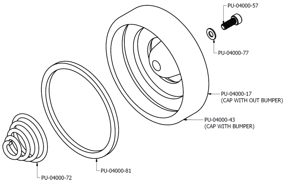
Figure 25: Air Cylinder Cap Assembly, (Part No. PU-04000-44), Exploded View
