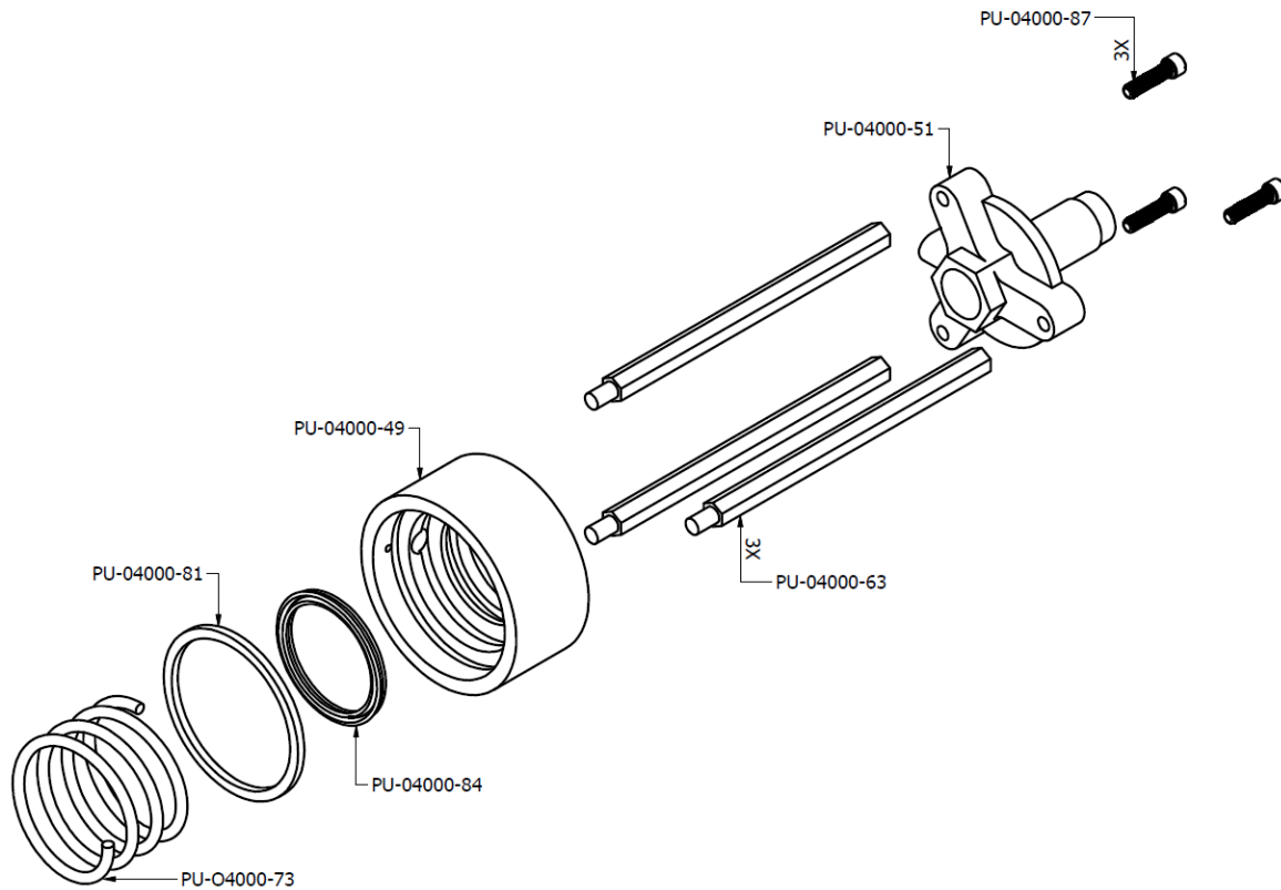
Figure 24: Air Motor to Pump Coupling Assembly, (Part No. PU-04000-23), Exploded View
