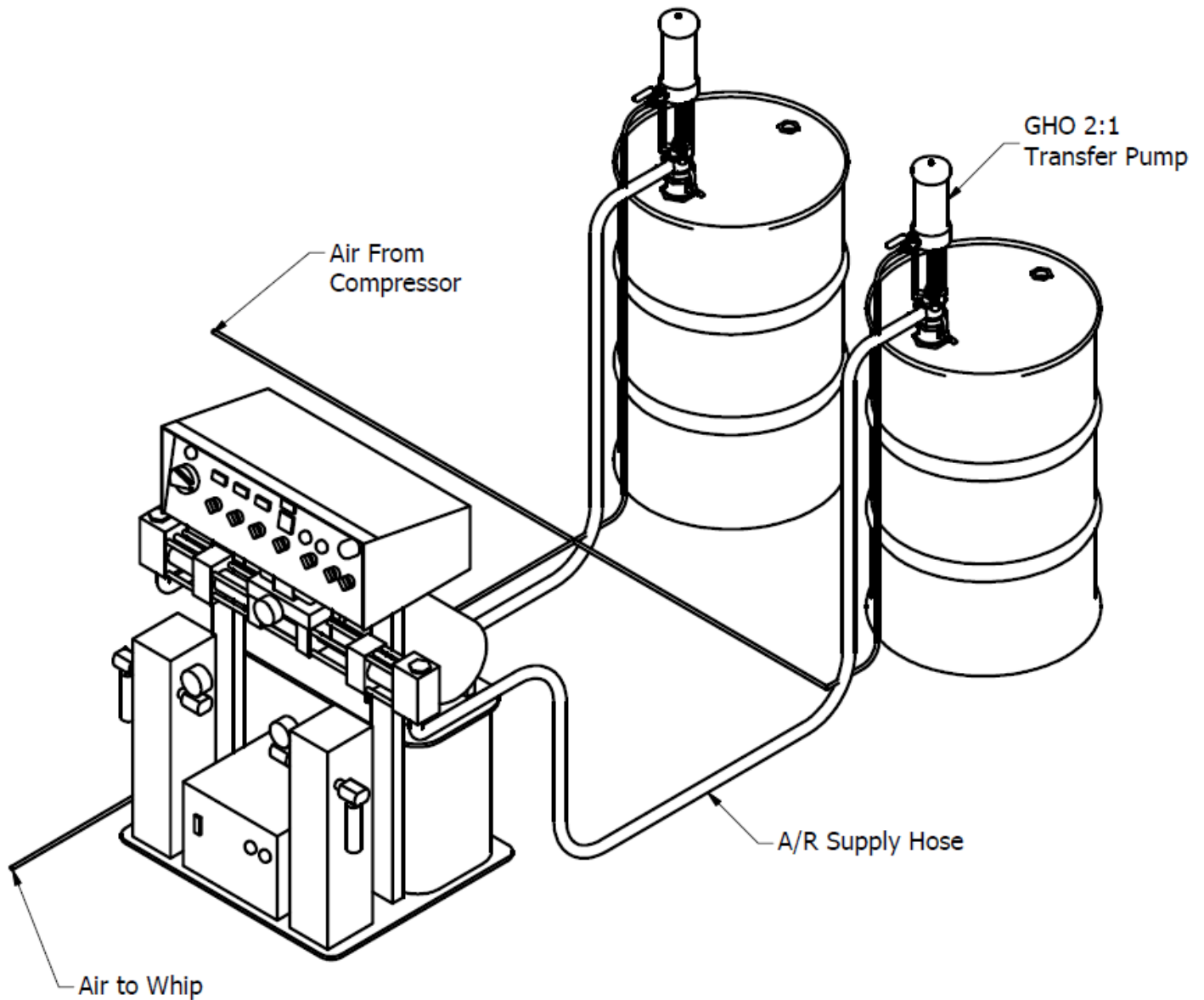
Figure 6: Typical Installation for Classic Hydraulic Proportioner
