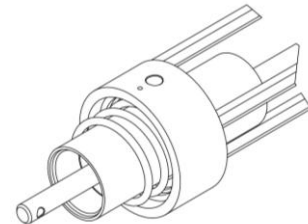
Figure 19: Remove Piston
