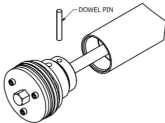
Figure 18: Dowel Pins
