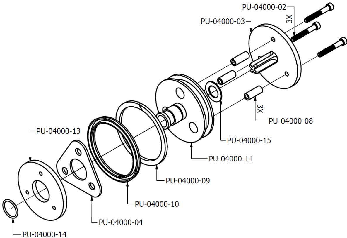
Figure 22: Air Motor Assembly, (Part No. PU-04000-01), Exploded View
