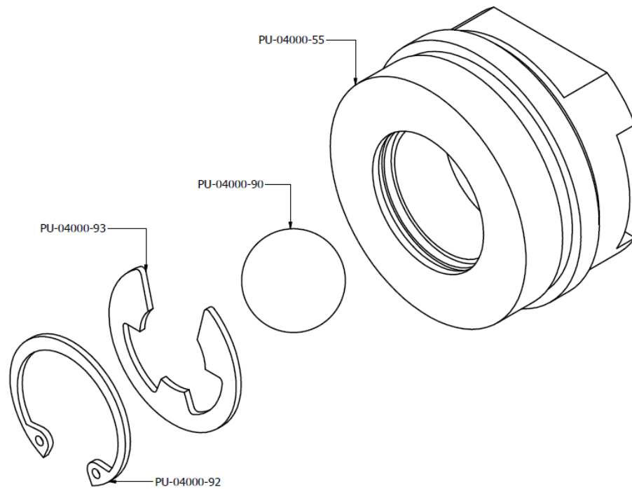
Figure 26: Foot Valve Assembly, (Part No. PU-04000-45), Exploded View
