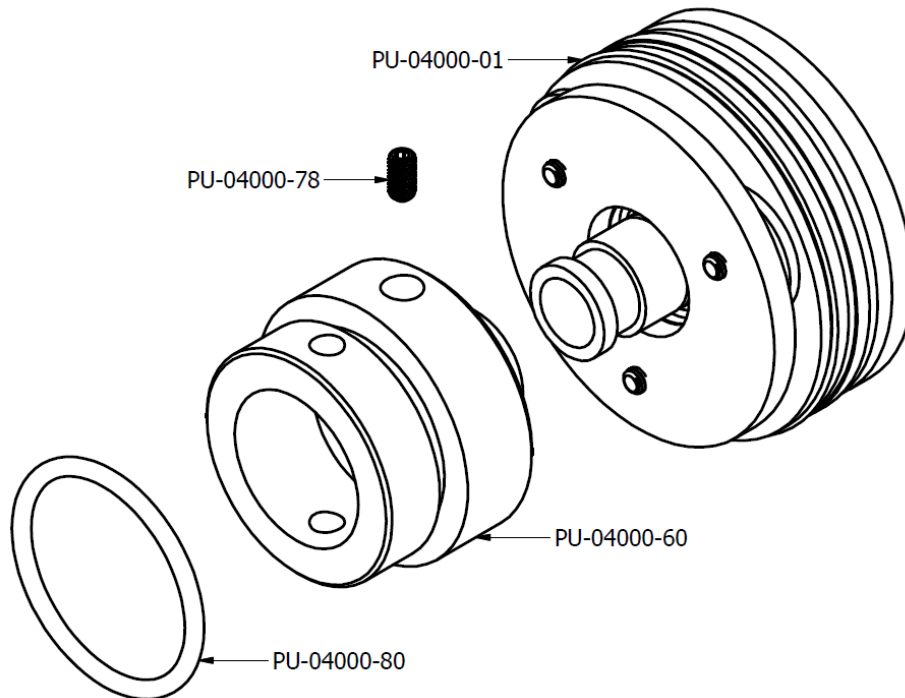
Figure 23: Air Motor and Plunger Top Assembly, (Part No. PU-04000-18), Exploded View
