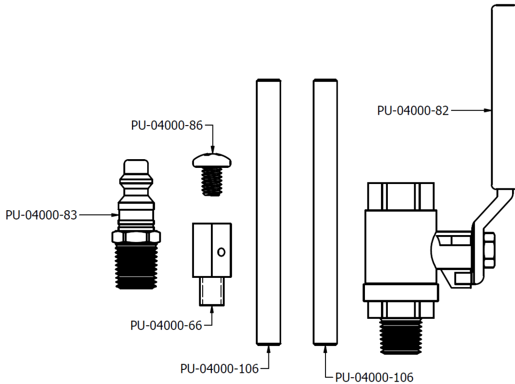
Figure 27: Tool Kit, (Part No. PU-04000-94), Exploded View
