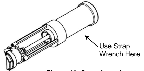
Figure 16: Strap Location
